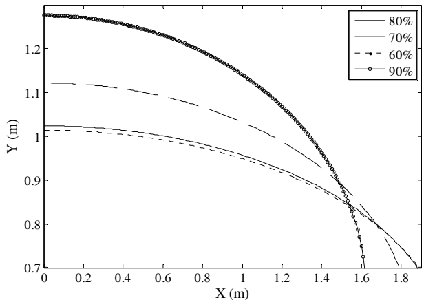
Fig13. Optimized elliptical cross-sections in different filling conditions
