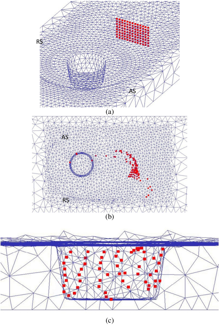
Fig12. (a) Initial position of points in front of tool which were picked for specification of overall material flow pattern, (b) and (c) final position of points.
