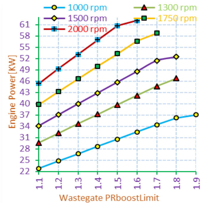
Fig13. Engine power VS. Pressure ratio.
