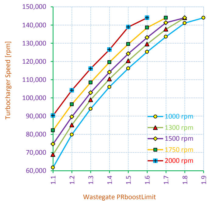
Fig11. Turbocharger speed VS. Limiting boost pressure ratio.
