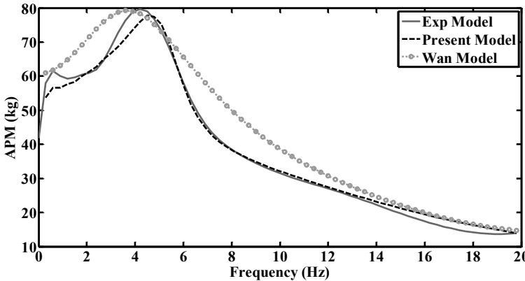
Fig8. . Apparent Mass responses
