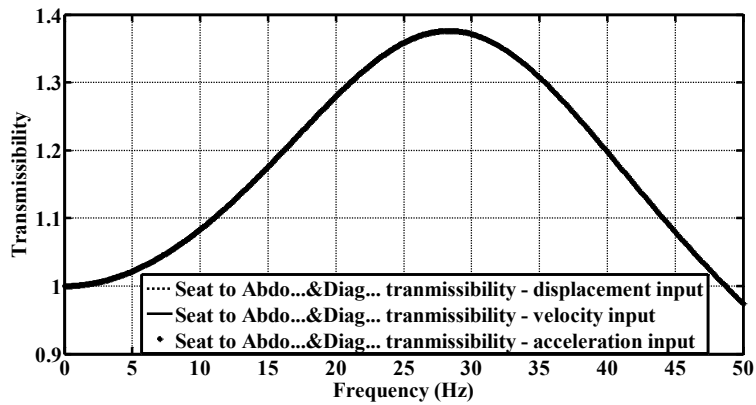
Fig28. Seat to abdomen &amp; diaphragm transmissibility
