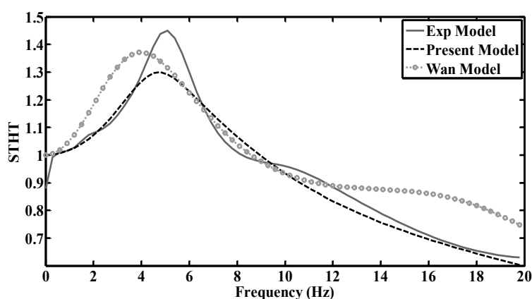
Fig6. Seat-To-Head Transmissibility responses
