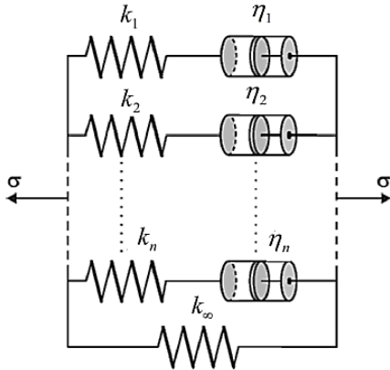
Fig2. Wicbert viscoelastic model
