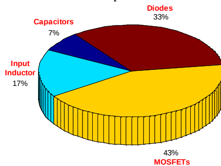
Figure 10: Percentage loss distribution of the proposed converter.
