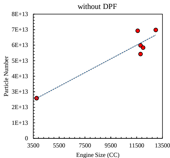
Figure 7: Relationship between engine displacement and emitted particulate matter in the absence of a particulate filter
