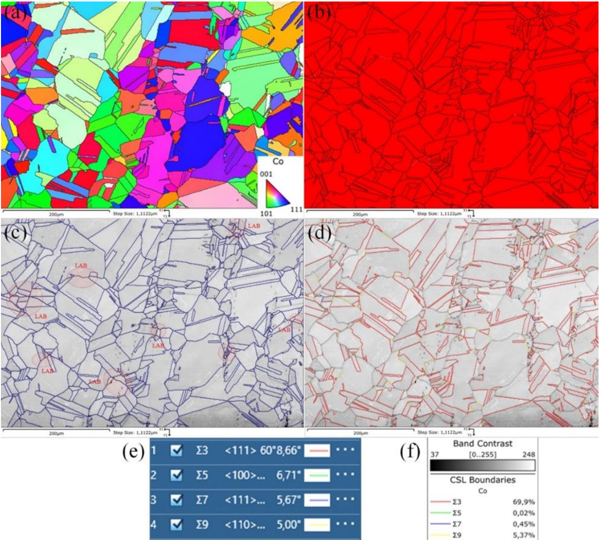
Fig. 4. EBSD maps of base metal: a) inverse pole figure (IPF) color, b) phase map, c) grain boundary distribution map d, e) coincidence site lattice and f) grain boundary distribution
